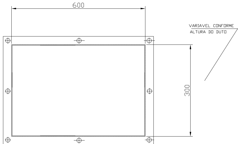
VISTA FRONTAL FUROS Ø 11mm.
